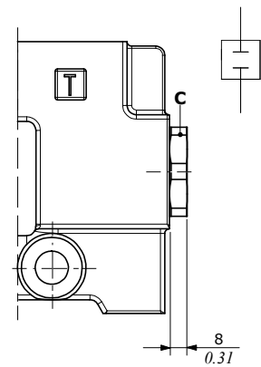
Relief valve blanking plug
