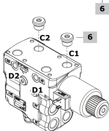
8ES2 control
