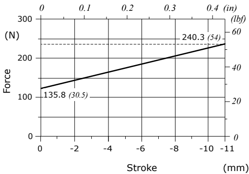
Force-Stroke diagram
