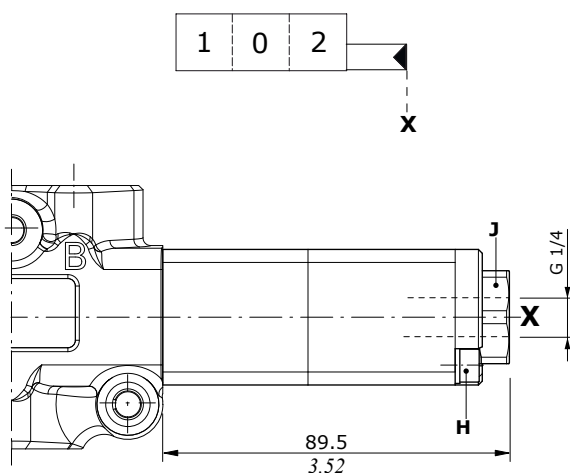
Type IA2 High pressure pilot
