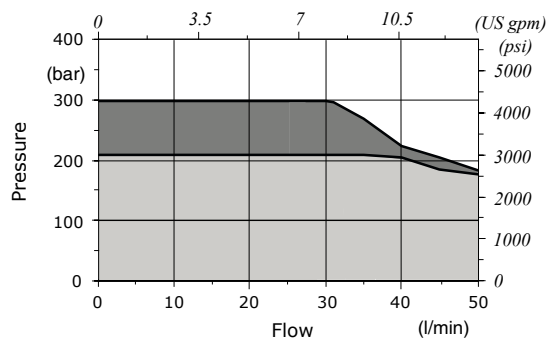
Minimum dynamic conditions (Supply = V_n - 10\% , coil at 70\text{ }^{\circ}\text{C} - 158\text{ }^{\circ}\text{F} )
