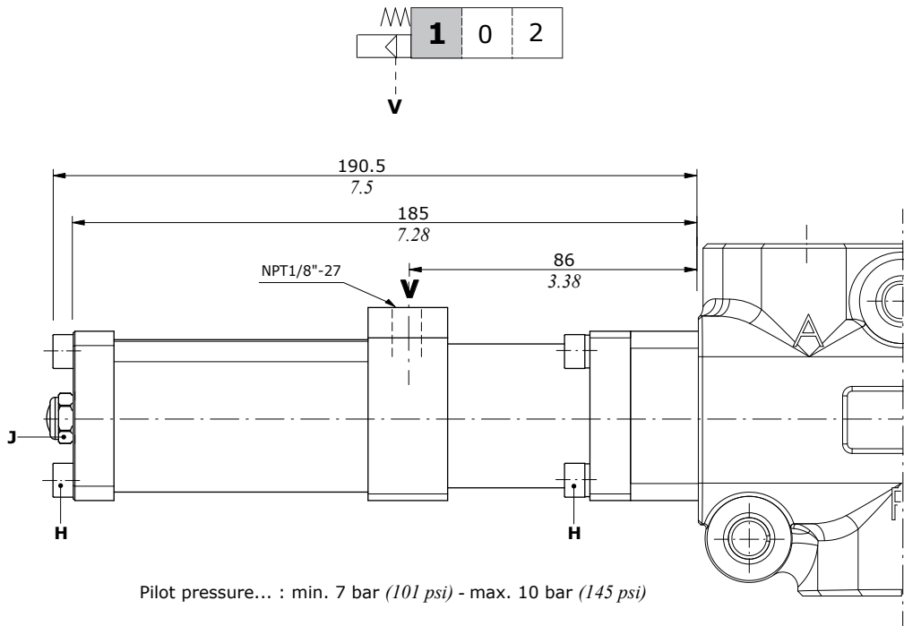
Type 17P Spring return in position 1
