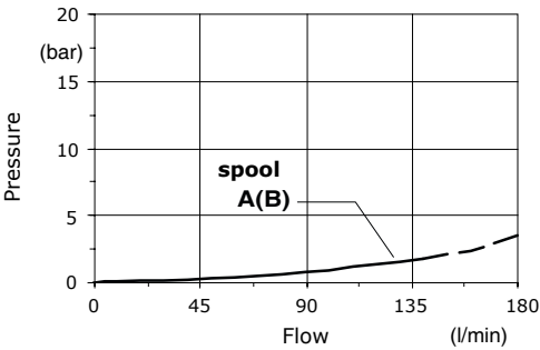
Pressure drop versus flow P → A(B)
