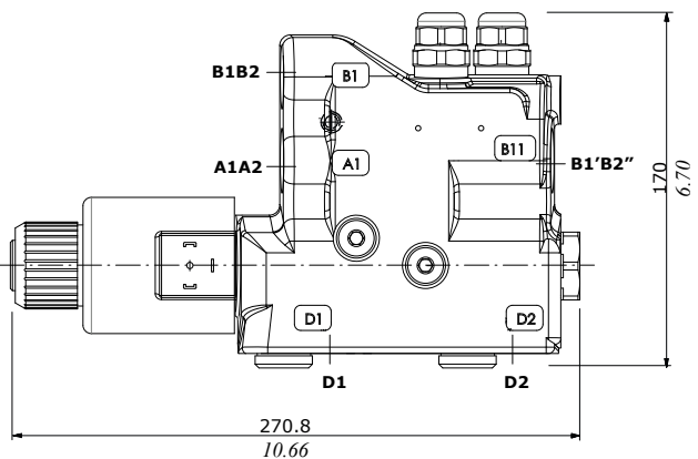
8ES2 configuration
