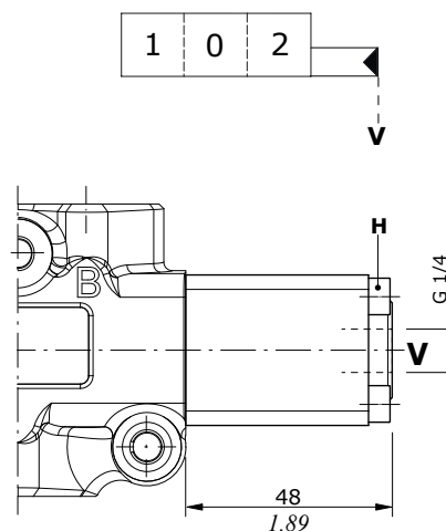
Type IB2 Low pressure pilot
