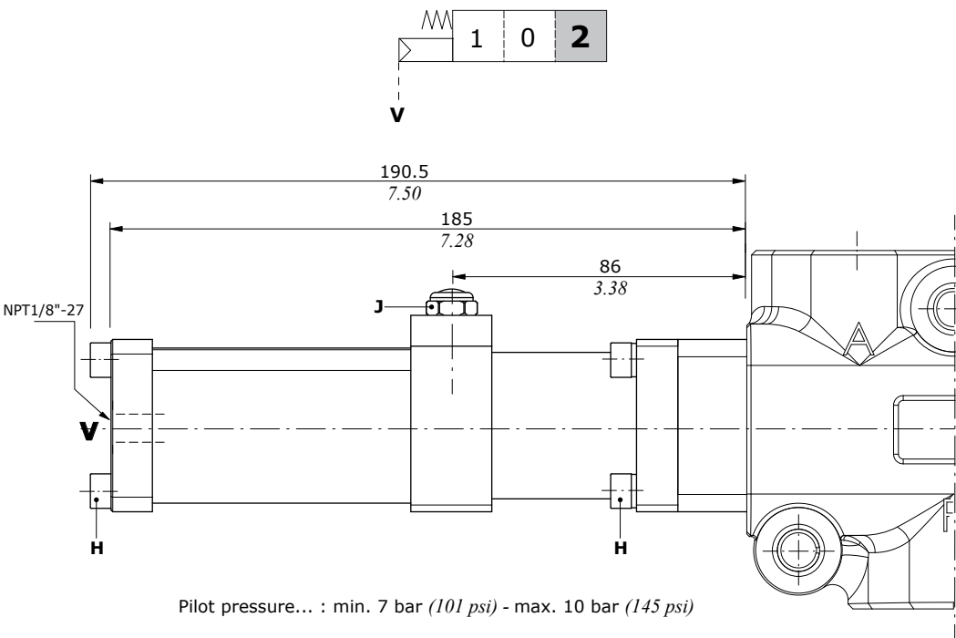
Type 18P Spring return in position 2
