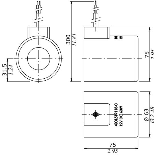
Flying leads
