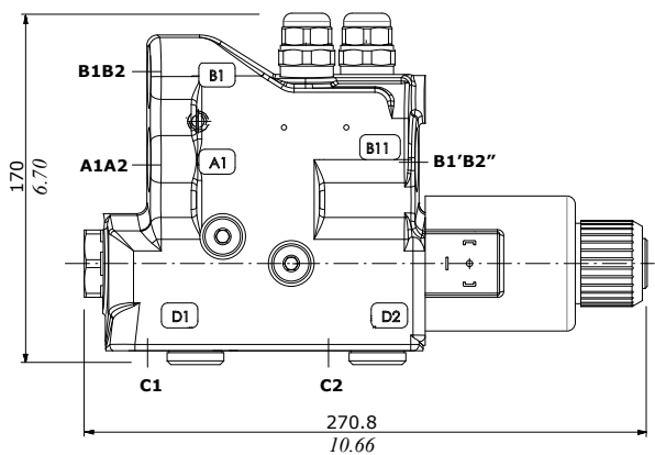
8ES1 configuration
