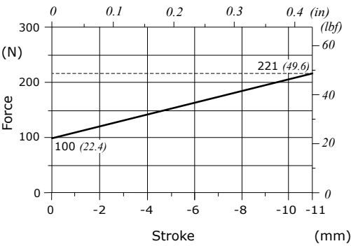
Force-Stroke diagram
