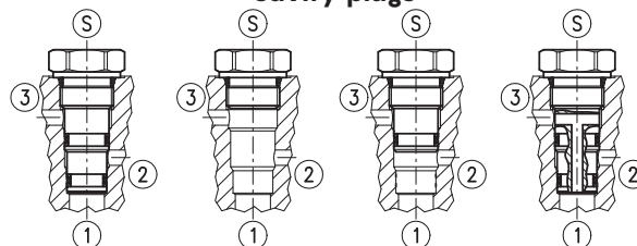
Cavity plugs
