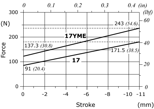
Force-Stroke diagram
