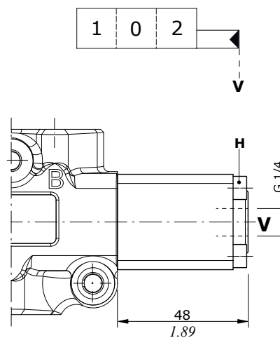
Type IB2 Low pressure pilot
