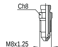
BORED BOLT WITH HOLE FOR BLEEDER SCREW REF. 12591
