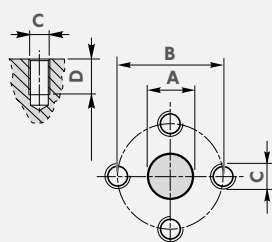
F: SAE J518-1 connection
