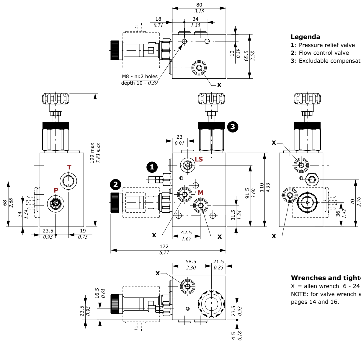
AN6 type for Open Center circuit
