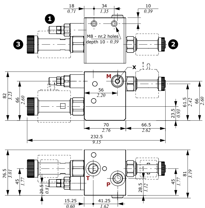
AN2B type with P and T ports open
