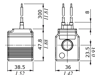
Flying leads
