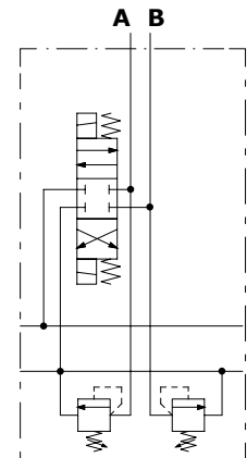
P type example (with spool 1)
