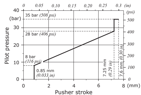
13IMP type: suggested pressure control curve on port VA: 073 type
