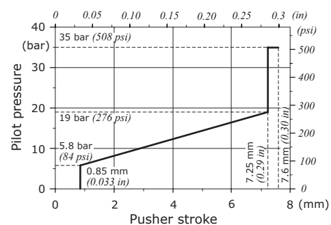
13IMP type: suggested pressure control curve on port VB: E073 type
