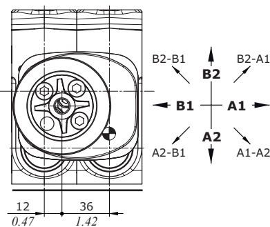
LCB4 configuration
