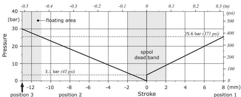
13IMOH type: Stroke vs. Pressure diagram
