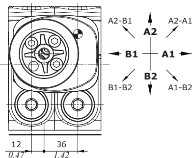
LCB4 configuration
