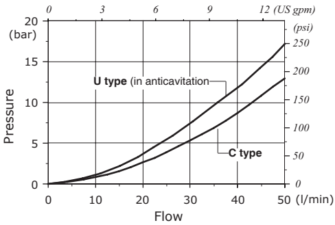
U and C types: pressure drops
