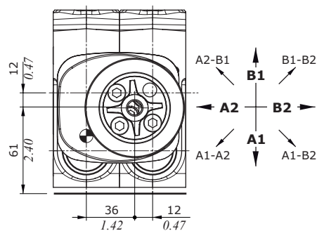
LCB3 configuration
