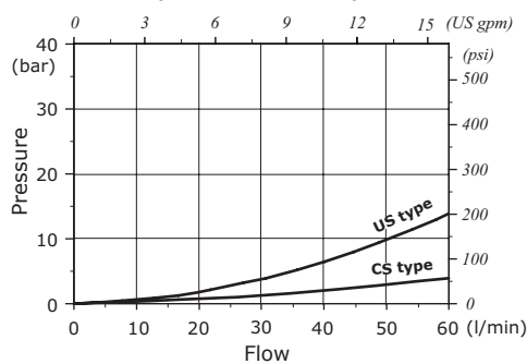
US-CS types, pressure drop (in anticavitation)
