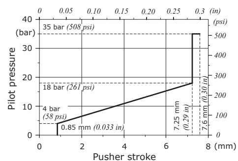
13IMOH type: suggested pressure control curve on port VB: 033 type
