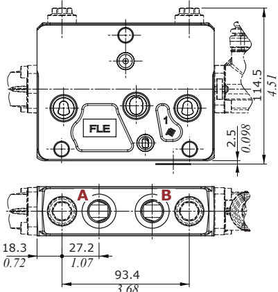
P type, for std or HP sections (G3/8 or G1/2 ports)
