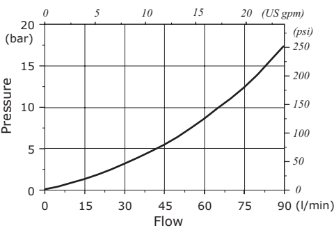
Pressure drop
