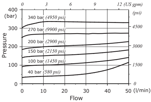
U type: setting example (10 l/min - 2.6 Us gpm)
