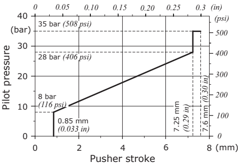
Suggested pressure control curve: 089 type
